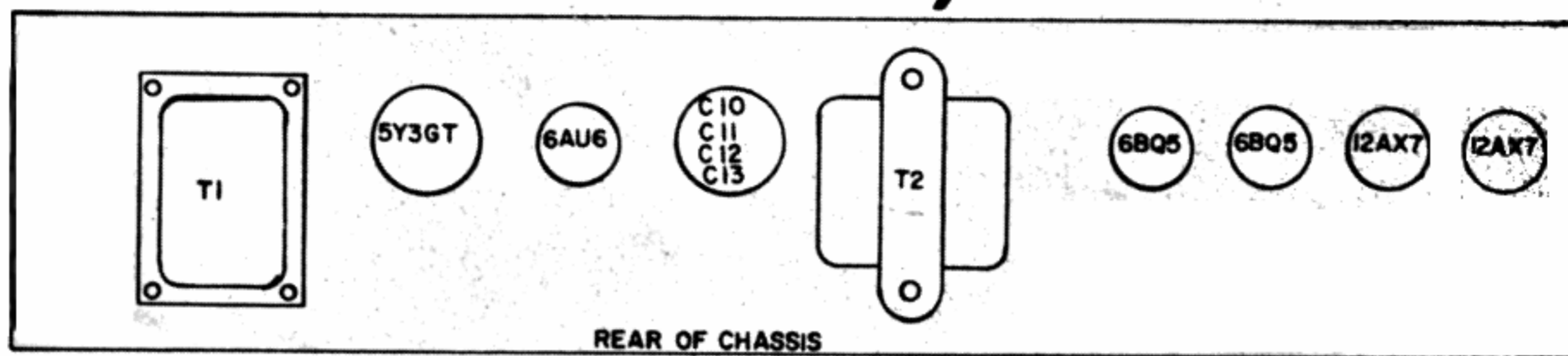
TUBE LAYOUT
