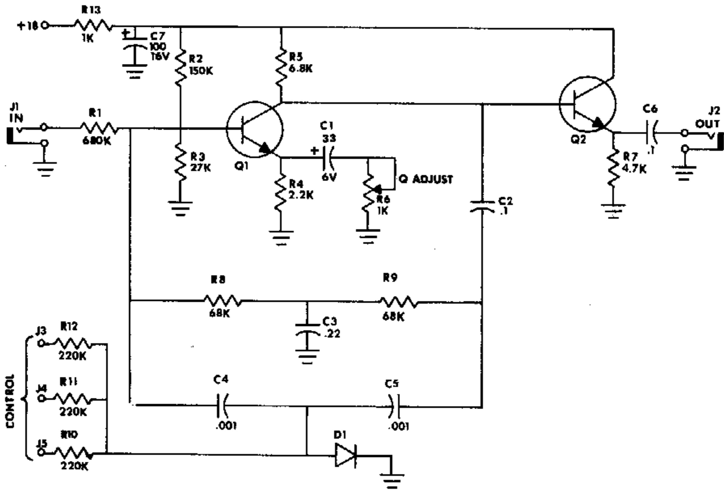
2720-3B Voltage Controlled Bandpass Filter
